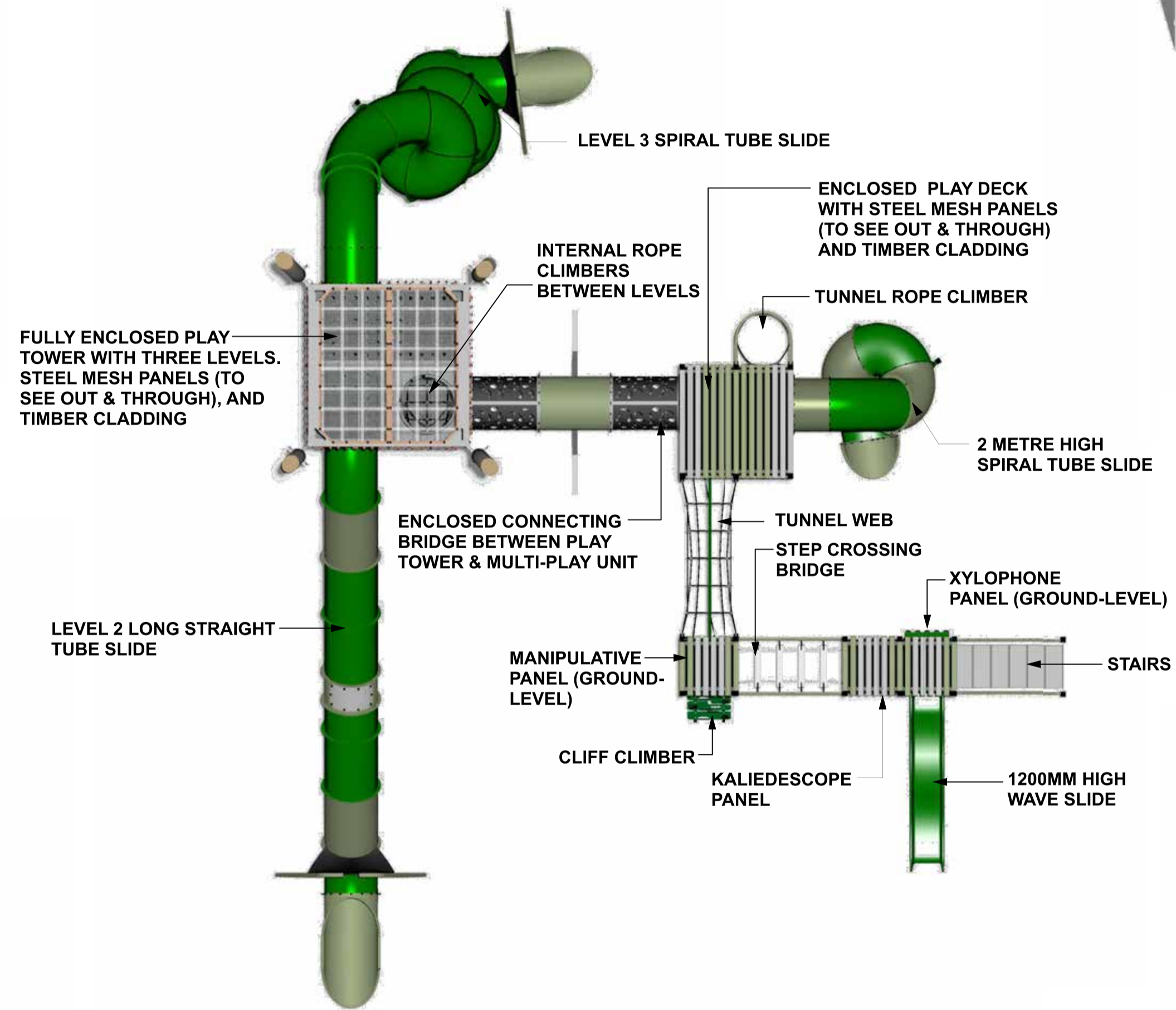
1 Play Tower & Multi-Play Unit - Detail Plan CD03 Not To Scale
